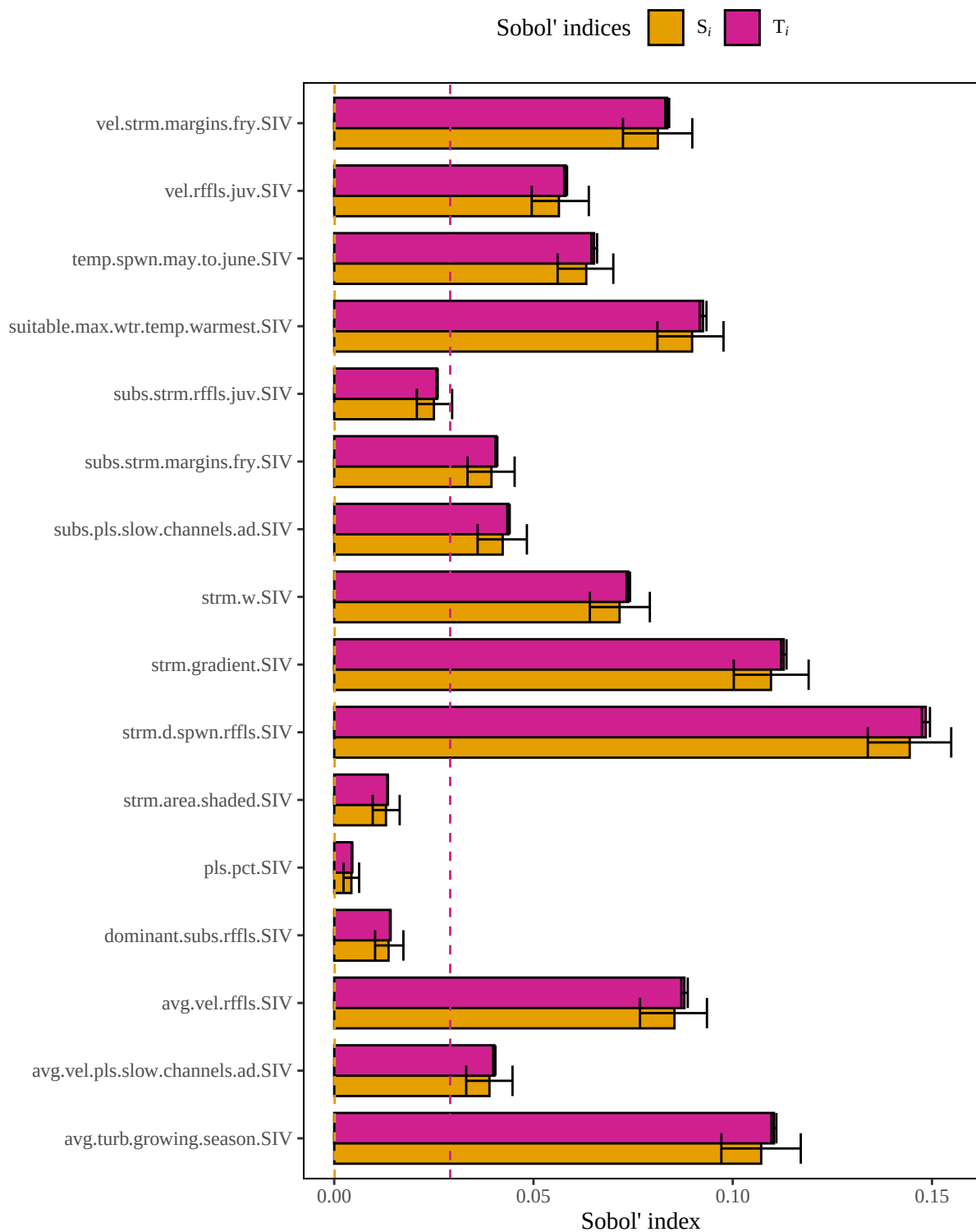
Figure 5. Results of a sensitivity analysis for the blacknosedaceRiv model based on a geometric mean structure. Dashed lines represent baseline numerical approximation error for S_i and T_i ( i.e. , dummy variables).
