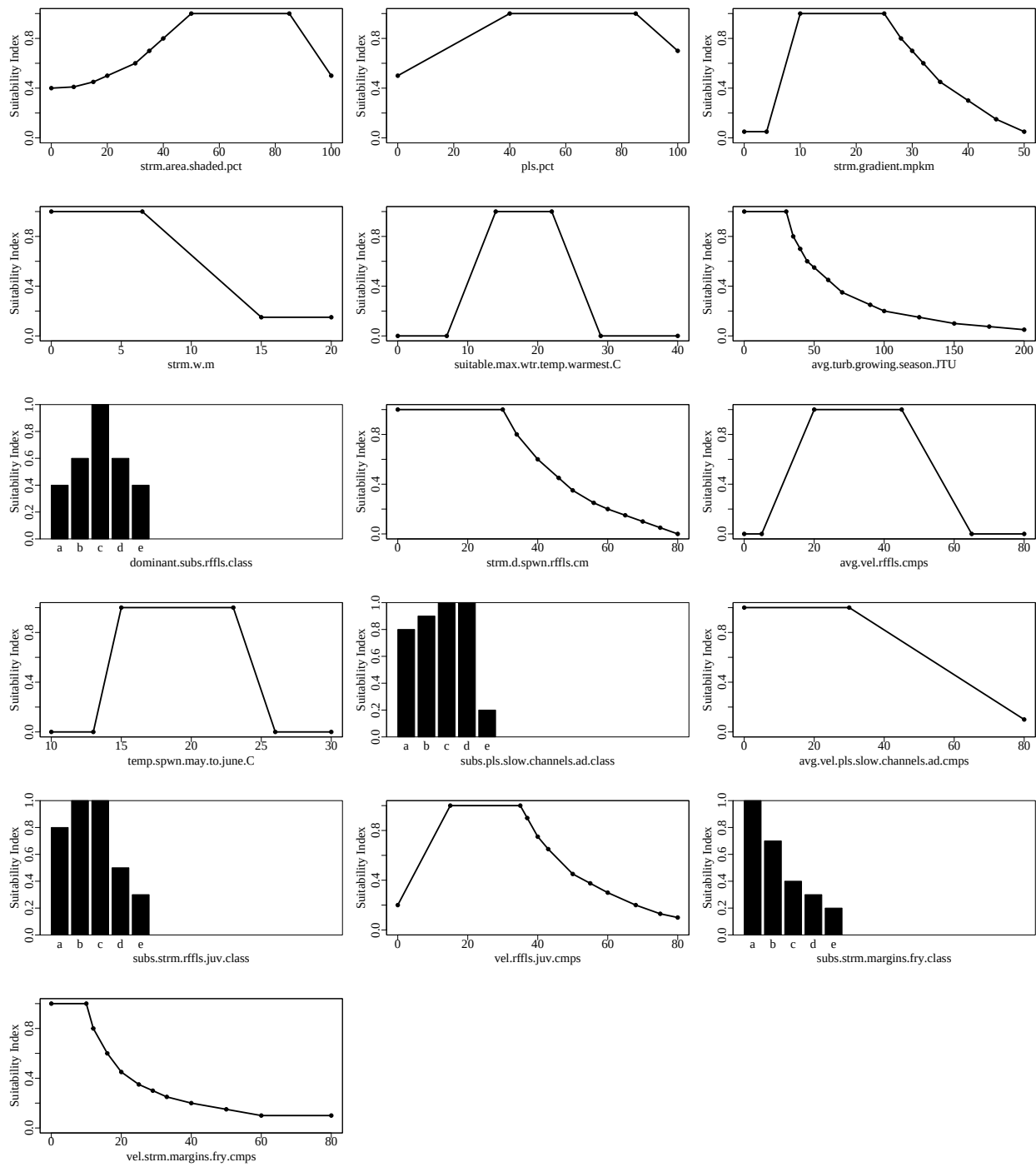
Figure 1. Suitability index graphs for variables included in the blacknosedaceRiv model in ecoest.
